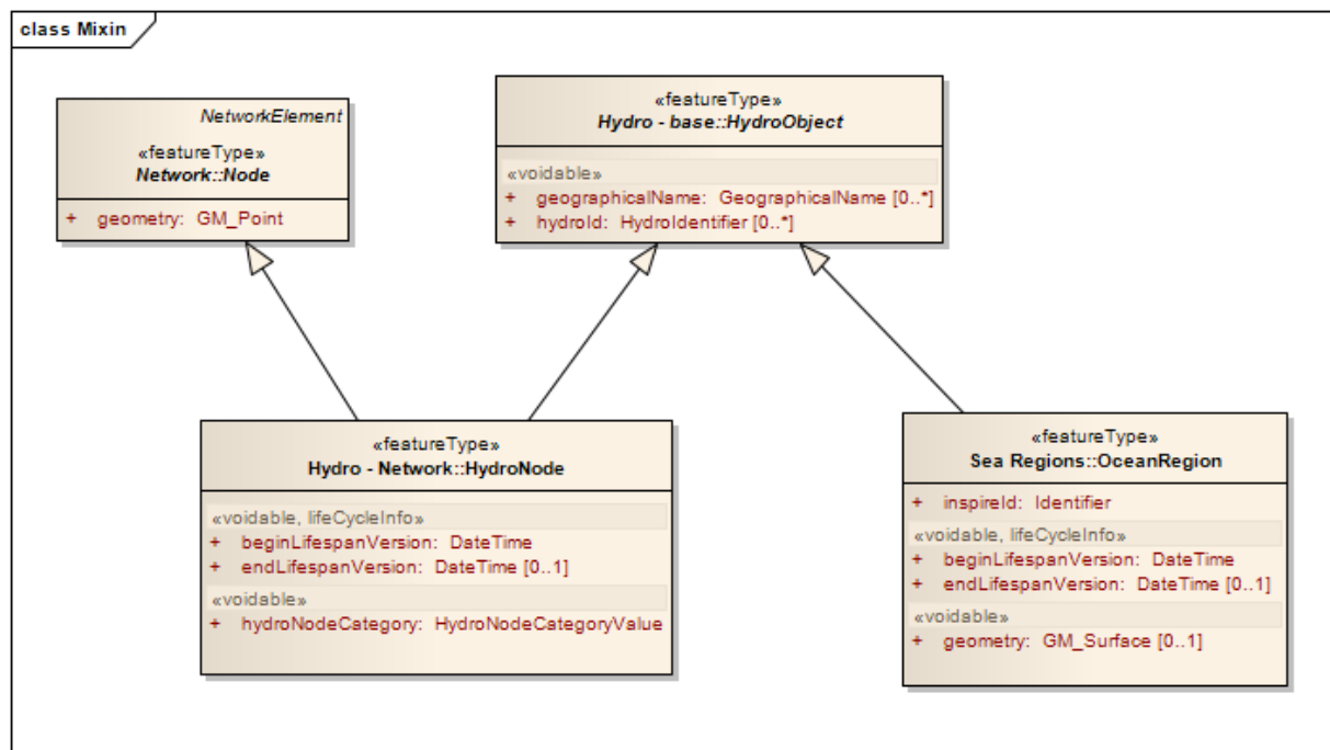
Figure 4 – Mixin example
