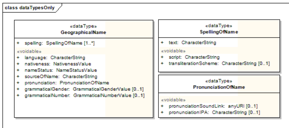
Figure 4 – UML class diagram: Data types
