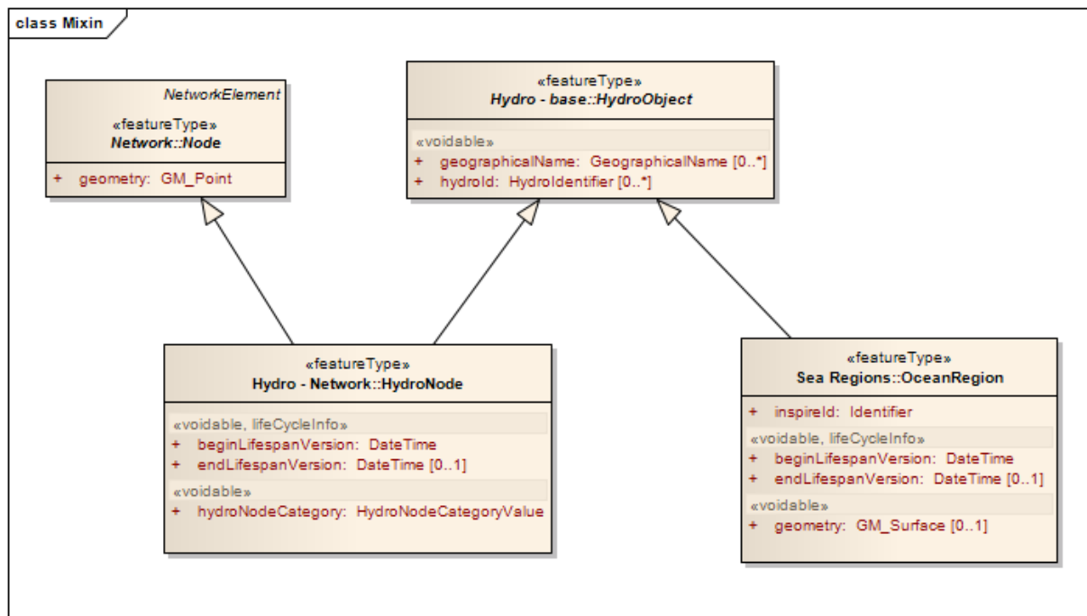
Figure 4 – Mixin example
